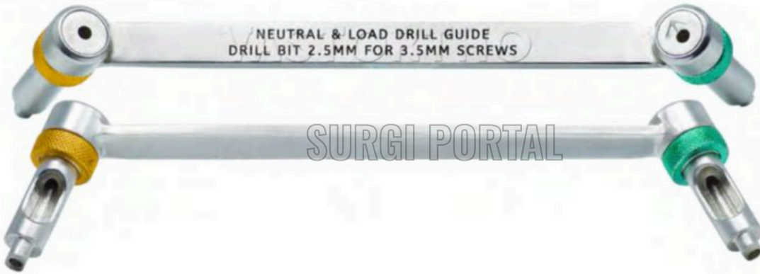
Drill Guide 3.5 mm for Neutral and Load Position
